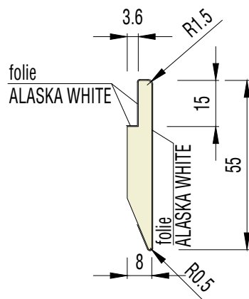
vkladka pro LED 5508
