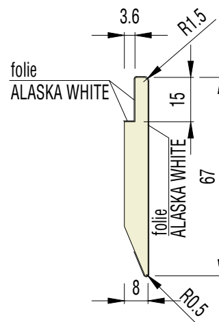
vkladka pro LED 6708
