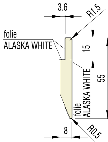
vkladka pro LED 5508
