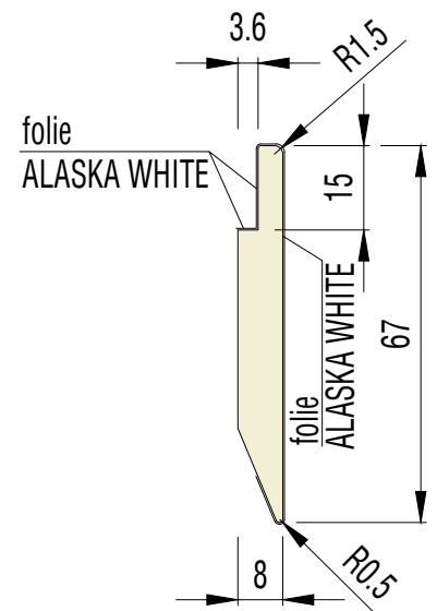
vkladka pro LED 6708
